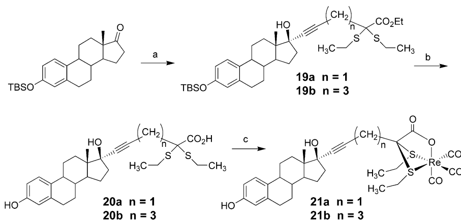
Scheme 6. Reagents and conditions (yield): (a) 16a or 16b , n\text{BuLi} , THF ( 19a 53%, 19b 46%); (b) \text{NaOH} , \text{H}_2\text{O} , \text{MeOH} ( 20a 65%, 20b 78%); (c) \text{Re}(\text{CO})_3^+ , \text{H}_2\text{O} ( 21a 29%, 21b 68%).
