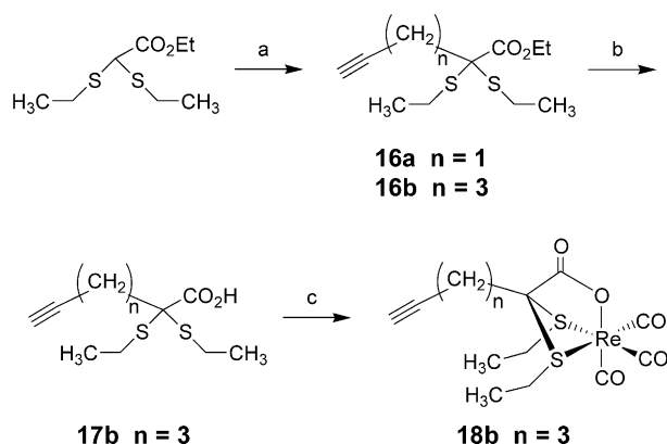
Scheme 5. Reagents and conditions (yield): (a) KOtBu, THF, propargyl bromide or 15 ( 16a 58%, 16b 57%); (b) NaOH, H 2 O, MeOH (90%); (c) Re(CO) 3 + , H 2 O (49%).
