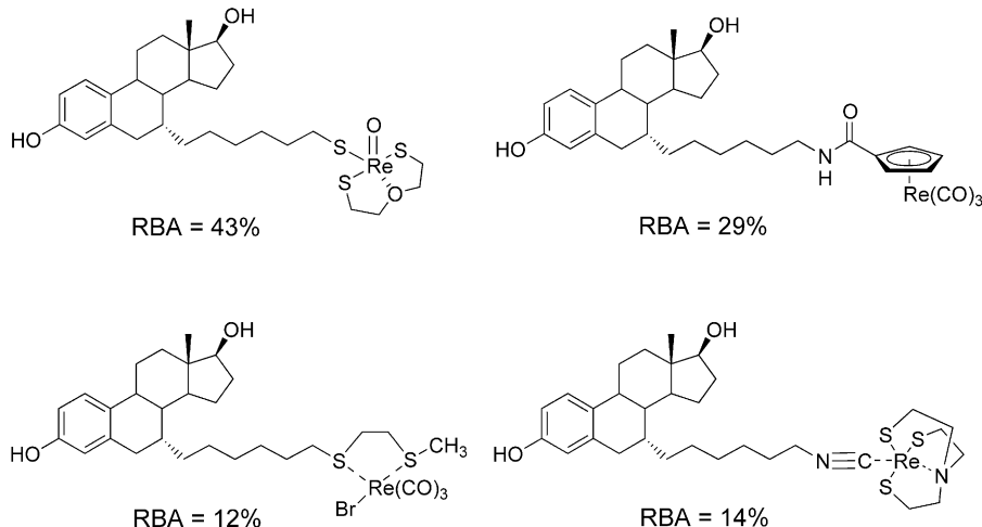
Figure 1. Representative examples of 7 \alpha -substituted estradiols with their corresponding relative binding affinity (RBA, estradiol = 100%).
