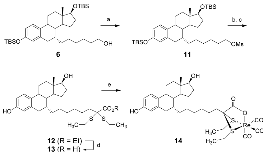
Scheme 4. Reagents and conditions (yield): (a) \text{MsCl} , \text{NEt}_3 , THF (quant); (b) (\text{CH}_3\text{CH}_2\text{S})_2\text{CHCO}_2\text{Et} , \text{KOtBu} , THF; (c) 40% HF, THF, \text{CH}_3\text{CN} (30% two steps); (d) \text{NaOH} , \text{H}_2\text{O} , MeOH (57%); (e) \text{Re}(\text{CO})_3^+ , \text{H}_2\text{O} (44%).
