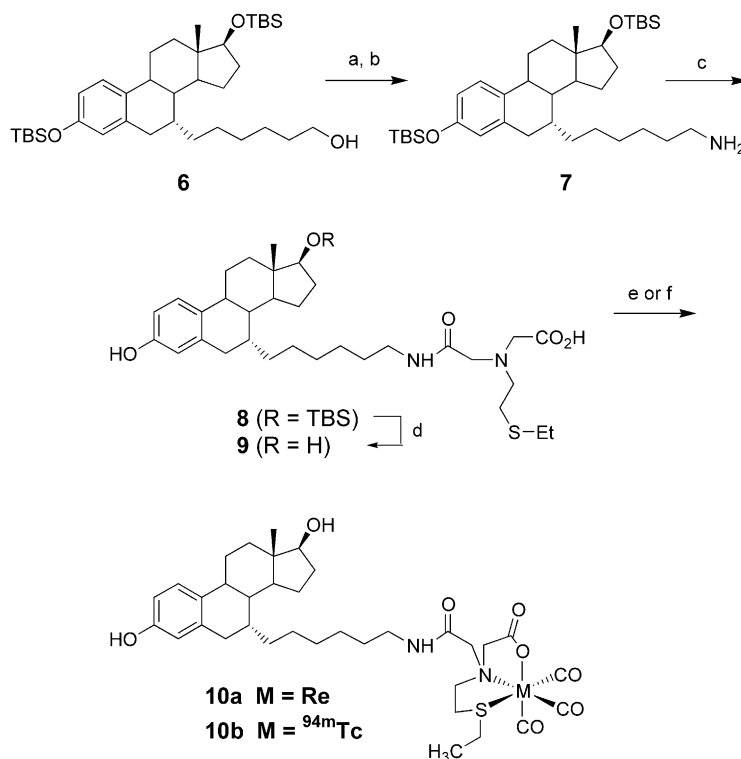
Scheme 3. Reagents and conditions (yield): (a) \text{PPh}_3 , DEAD, phthalimide, THF; 19 (b) \text{NH}_2\text{NH}_2 , DME, EtOH; 19 (c) 1 , EDC, DMAP, DMF, \text{CH}_2\text{Cl}_2 (40%); (d) 40% HF, THF, \text{CH}_3\text{CN} (quant); (e) \text{Re}(\text{CO})_3^+ , \text{H}_2\text{O} (48%); (f) ^{94m}\text{Tc}(\text{CO})_3^+ , \text{H}_2\text{O} .
