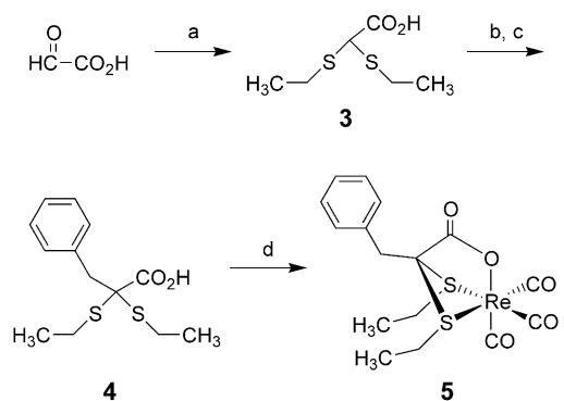
Scheme 2. Reagents and conditions (yield): (a) EtSH, TsOH, benzene (93%); (b) nBuLi, THF; (c) BnBr, THF (68%); (d) \text{Re}(\text{CO})_3^+ , \text{H}_2\text{O} (79%).
