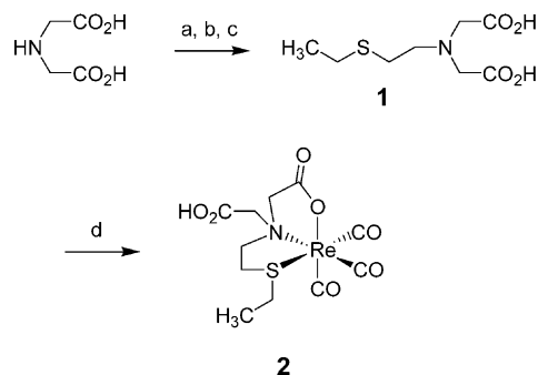
Scheme 1. Reagents and conditions (yield): (a) NaOH, ClCH 2 CH 2 SCH 2 CH 3 , H 2 O, EtOH; (b) BaCl 2 , H 2 O; (c) H 2 SO 4 , H 2 O (46% three steps); (d) Re(CO) 3 + , H 2 O (88%).
